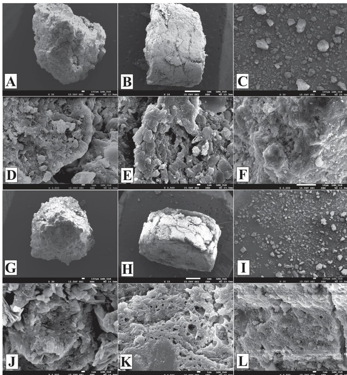
Figure 6. Scanning electron microscopy images (SEM) of the BBFs granules, pellets and powders. A, B and C: BBF-KCl in the form of granules (with 30x magnification), pellets (with 15x magnification) and powder (with 30x magnification), respectively; D, E and F: BBF-KCl in the form of granules, pellets and powder, respectively, with 3500x magnification; G, H and I: BBF-K 2 SO 4 granules (with 30x magnification), pellets (with 15x magnification) and powder (with 30x magnification), respectively; J, K and L: BBF-K 2 SO 4 in the form of granules, pellets and powder, respectively, with 3500x magnification.
